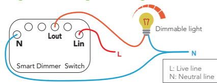
Diagram 1: For light dimming
